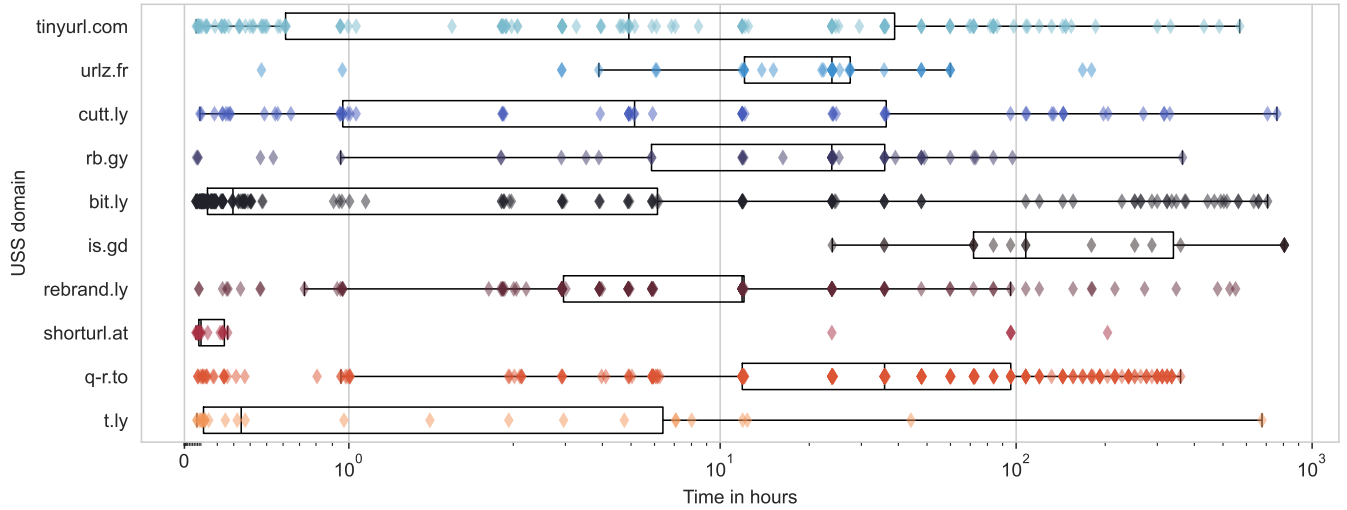
Fig. 5. Uptimes of abused short URLs. Boxplots represent the time elapsed between the short URL being blocklisted and deactivated. The data in the range from 0 to 1 is in the linear scale, while the rest is logarithmic. The left and right ends of the box mark 25th and 75th percentiles, and the line inside is the 50th percentile. We only have few samples from t.ly , is.gd , and shorturl.at so the results are not fully representative of the service uptimes.
