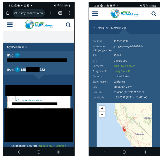
(a) The (public) IP address of G (b) Lookup of 66.249.81.238.
