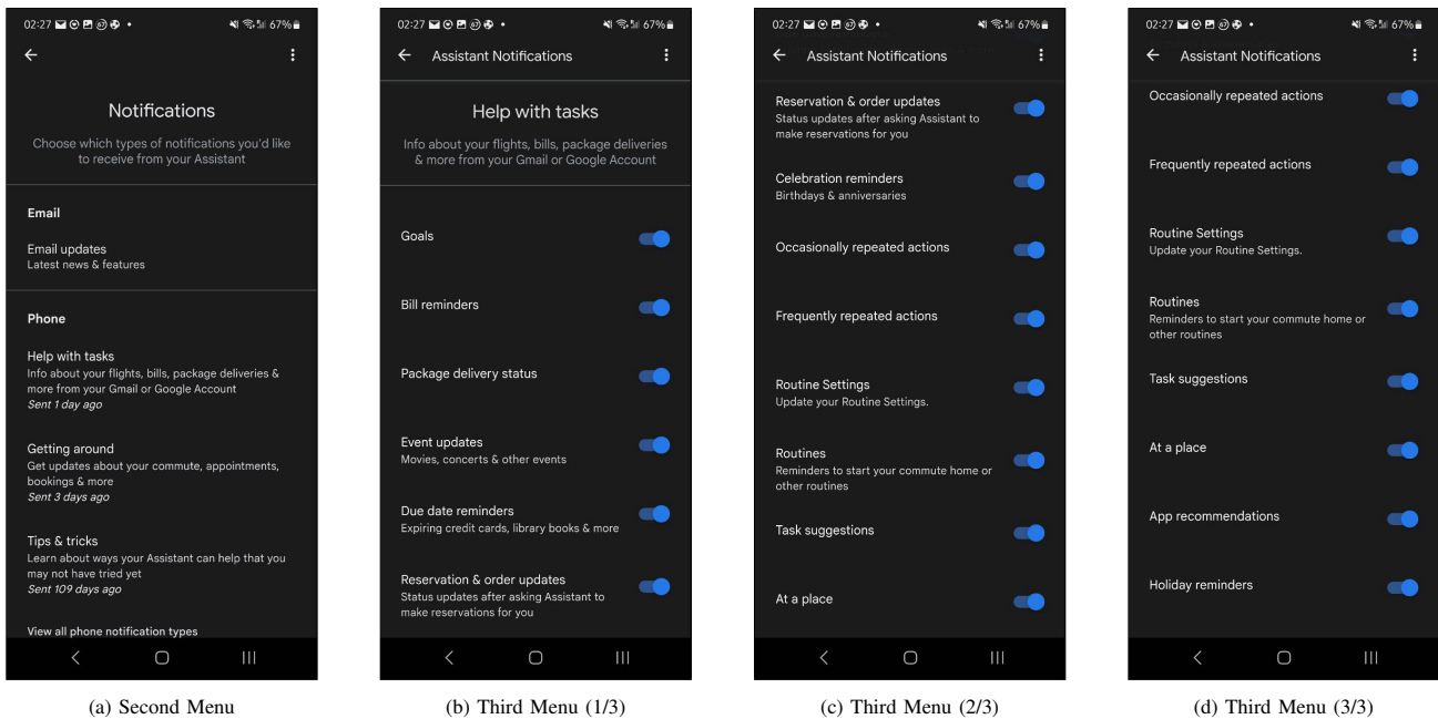
Fig. 9: Follow-up menus (from G's Samsung S23) pertaining to the "Google Assistant" options. After opening the "Notification" submenu (from Fig. 8c), we are first shown the tab in Fig. 9a. Then, after tapping on "Help with Tasks", we are shown a submenu having 15 options (Figs. 9b to 9d), all enabled by default. To prevent exploitation of the vulnerability discussed in this paper, one could theoretically opt-out from the "Due Date Reminders".
